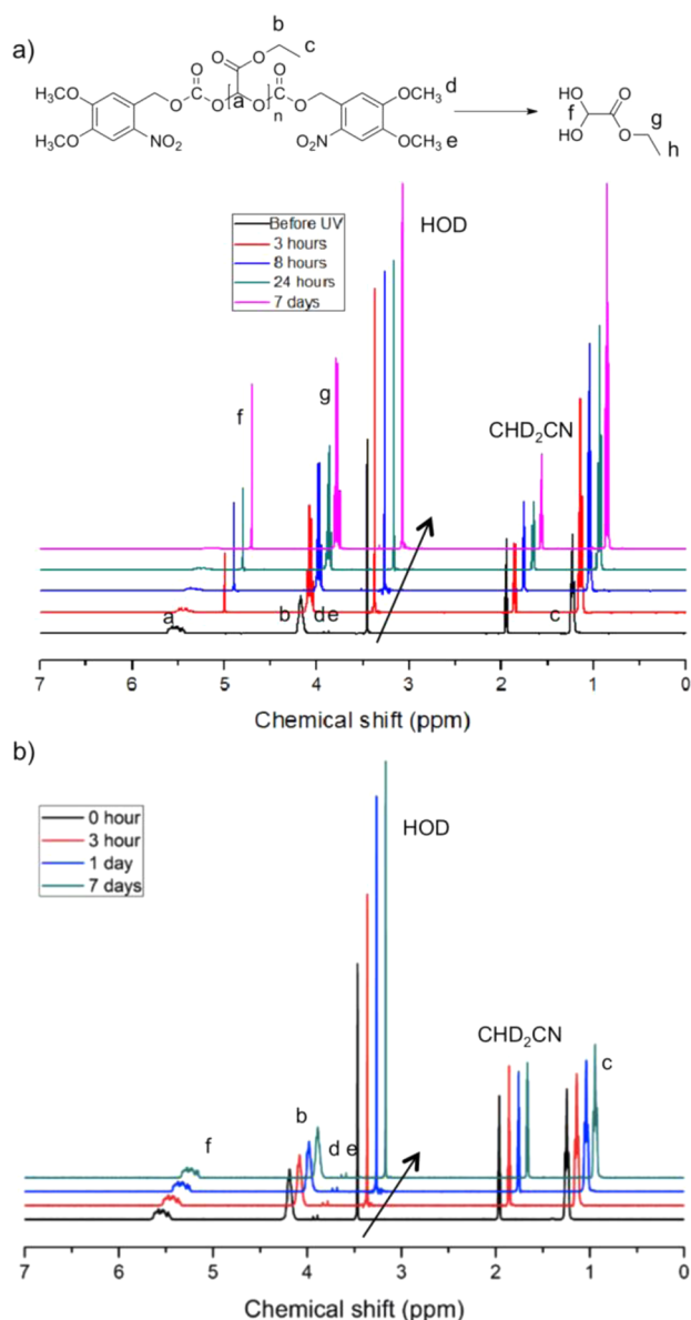
Figure 1. 1 H NMR spectra of PETg 4: (a) after UV irradiation and (b) without UV irradiation, following incubation in 9:1 CD 3 CN:D 2 O at 21 °C for varying time periods. Spectra are offset to allow the progression over time to be clearly observed. Additional spectral details are shown in Supporting Information Figures S48 and S49.
